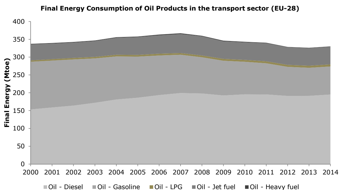
Figure 131: Final energy consumption of oil products in the EU-28 transport sector, 2000-2014. Source: Eurostat
