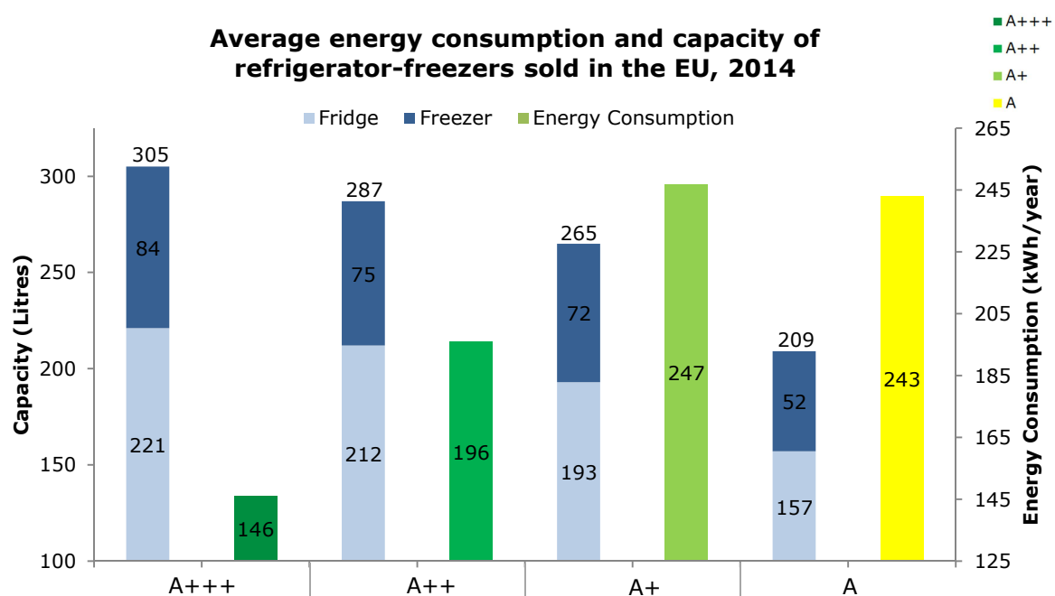
Figure 76: Average energy consumption and volume of refrigerator-freezers sold per efficiency class in the EU (21 countries), 2014. Source: topten.eu from GfK [18]
