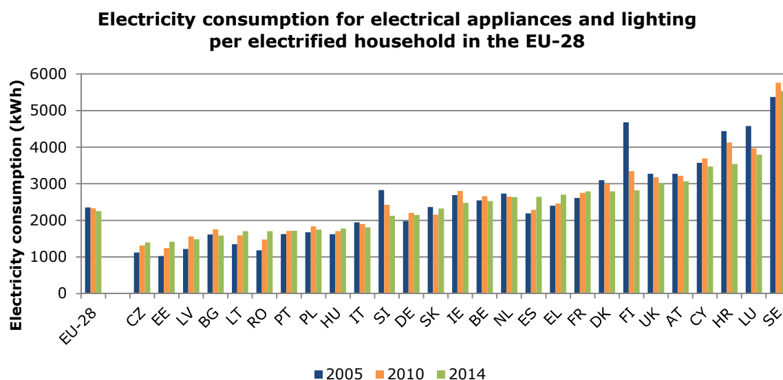
Figure 55: Electricity consumption for electrical appliances and lighting per electrified household in the EU-28, 2005, 2010 and 2014 62 . Source: Enerdata
