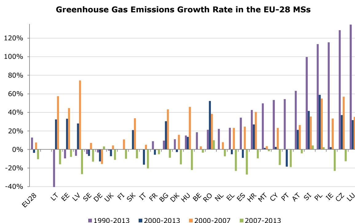
Figure 170: Greenhouse gas emissions growth rate in the EU-28 Member States; 1990-2013, 2000-2013, 2000-2007 and 2007-2013. Source: EEA
