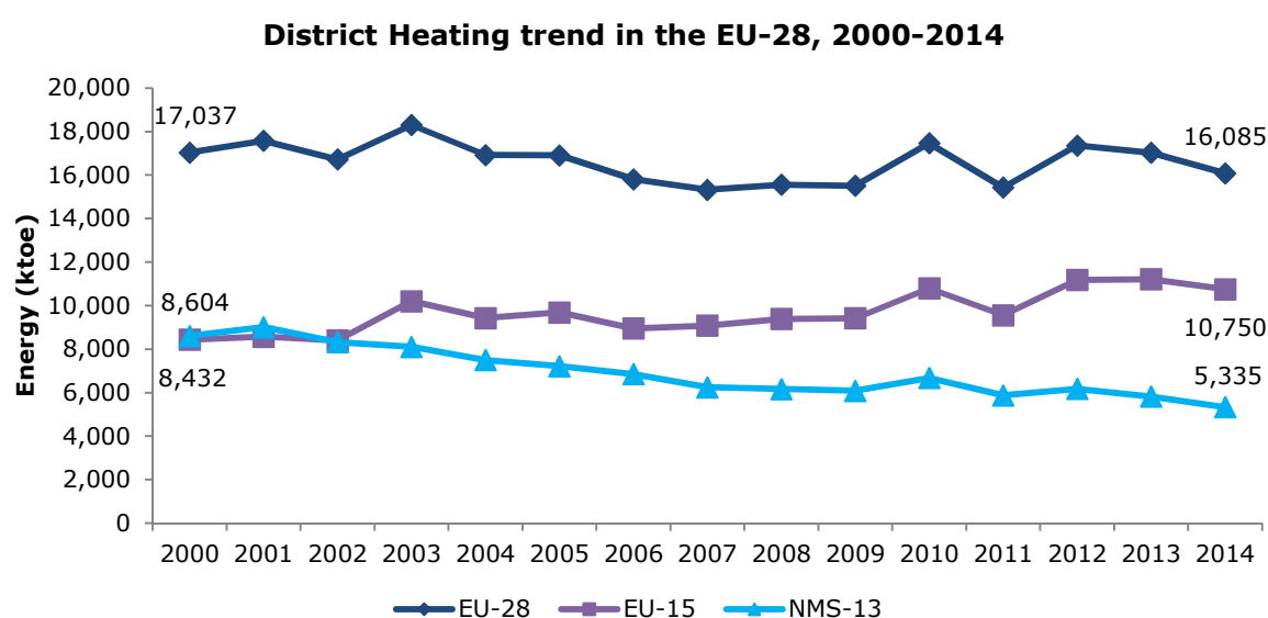
Figure 65: District heating plants supply (output production) trends in the EU28, 2000-2014. Source: Eurostat
