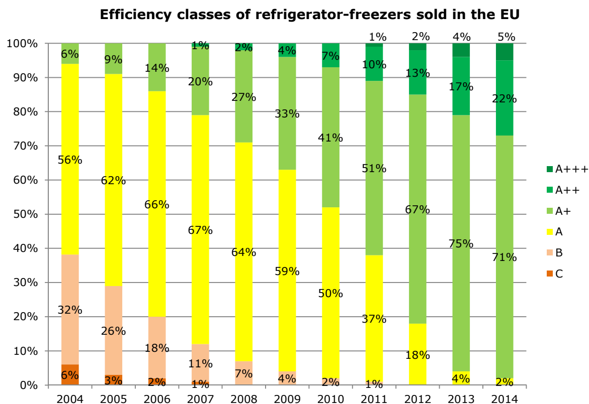
Figure 73: Energy efficiency classes of refrigerators-freezers in the EU (21 countries), 2004-2014. Source: topten.eu from GfK [17]
