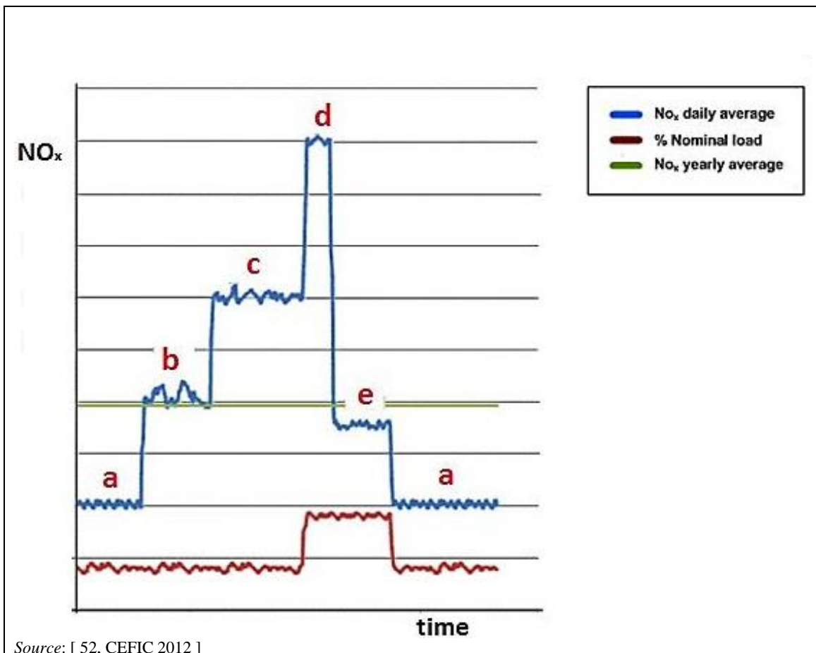
Figure 8.4: \text{NO}_x emissions pattern as a function of the daily operation of a utility boiler not fitted with end-of-pipe measures (values are not taken from real installations)
