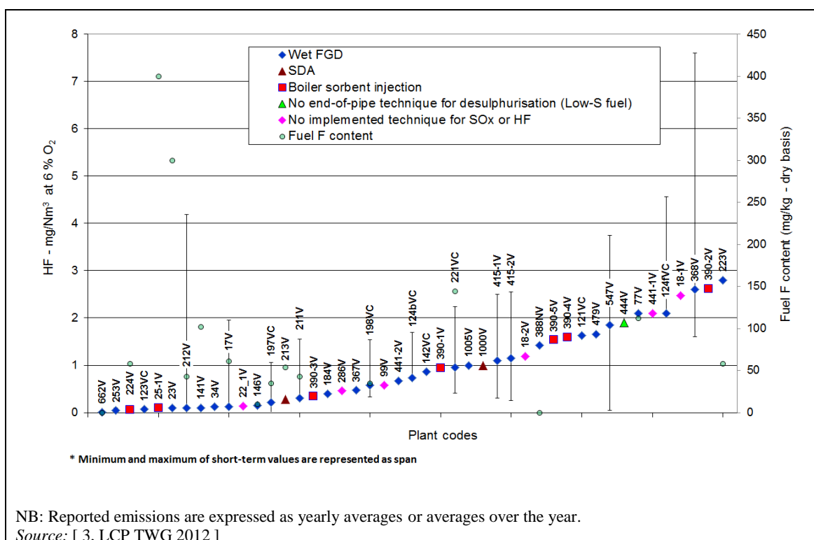
Figure 5.35: HF emissions from well-performing coal- and/or lignite-fired plants of > 100 \text{ MW}_{\text{th}}
