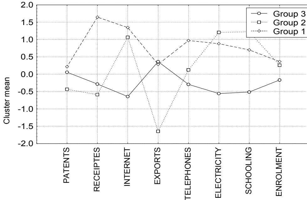
Figure 3.4. Plot of means for each cluster in the technology achievement case study. Type: k -means clustering (standardized data).
