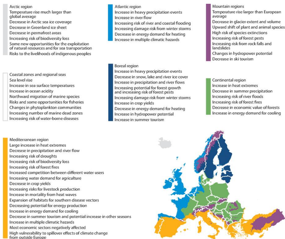
Figure 4. Key observed and projected climate change and impacts for the main biogeographical regions in Europe (EEA, 2016) (71)
