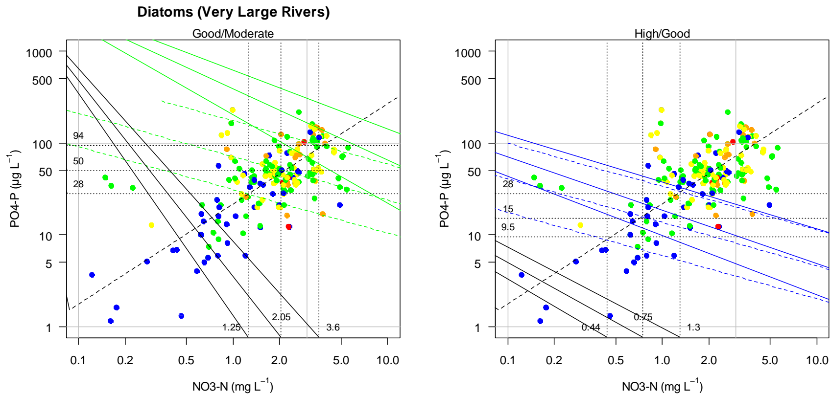
Figure 6-105 Relationship between mean ortho-P and nitrate N, points coloured by WFD class for phyto-benthos in very large rivers (Type R-L). Dotted lines contours of predicted TN & ortho-P concentration when national phyto-benthos ICM is at a) good/moderate boundary (green lines) and b) high good boundary, dotted lines show \pm 25^{\text{th}} & 75^{\text{th}} residuals of prediction. Horizontal & vertical lines show intersection with RMA regression of observed ortho-P and nitrate N showing boundary values.
