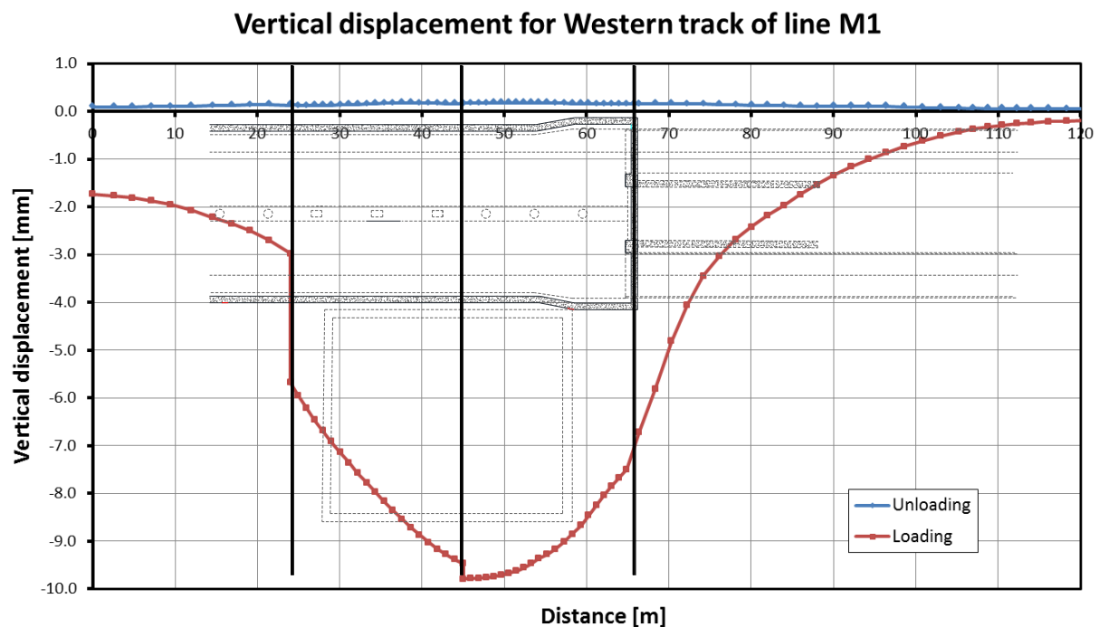
Figure A3. An example of displacement profile for a track bed of a metro line at different stages of a construction of a neighbouring building (modified after Bogusz and Godlewski, 2017b).
