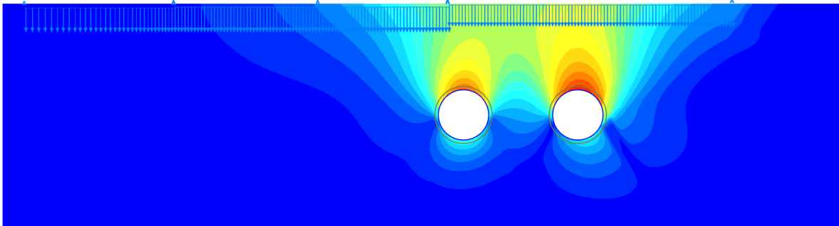
Figure A1. Example of map of predicted displacements caused by twin tunnels (TBM - EPB) constructed underneath existing buildings, simplified as distributed loads) (figure courtesy of W. Bogusz)
