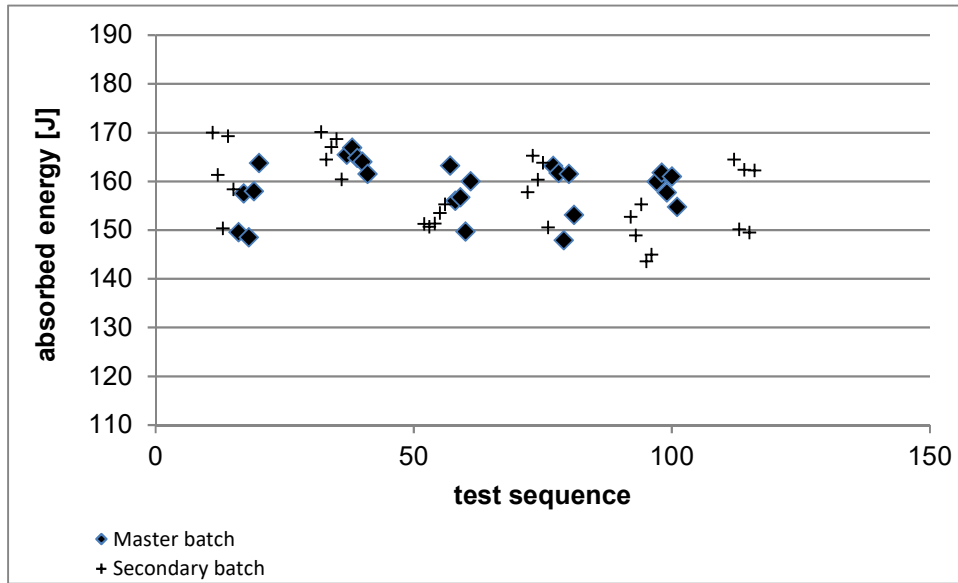
Figure 3: Absorbed energy values of 30 test pieces of ERM-FA415ao, compared with 25 test pieces of ERM-FA415s; data are displayed in the actual test sequence.
