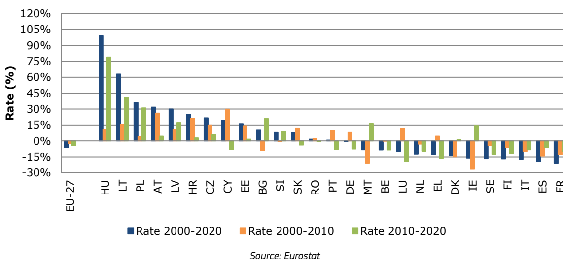
Figure 147: Industry sector: annual final electricity consumption rates in the EU-27; 2000-2020, 2000-2010 and 2010-2020
