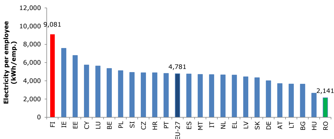
Figure 86: Annual electricity consumption per employee in the tertiary sector in the EU-27, 2020
