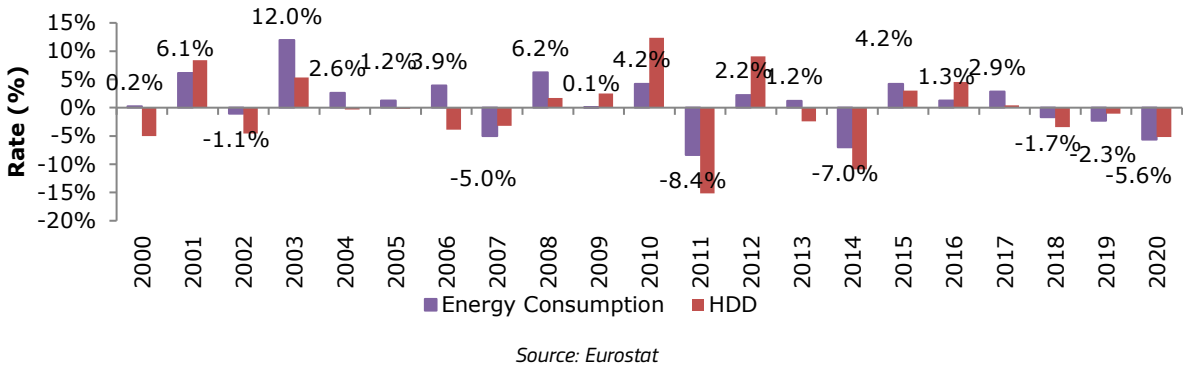
Figure 77: Tertiary final energy consumption and Heating Degree Days annual consumption rates in the EU-27, 2000-2020
