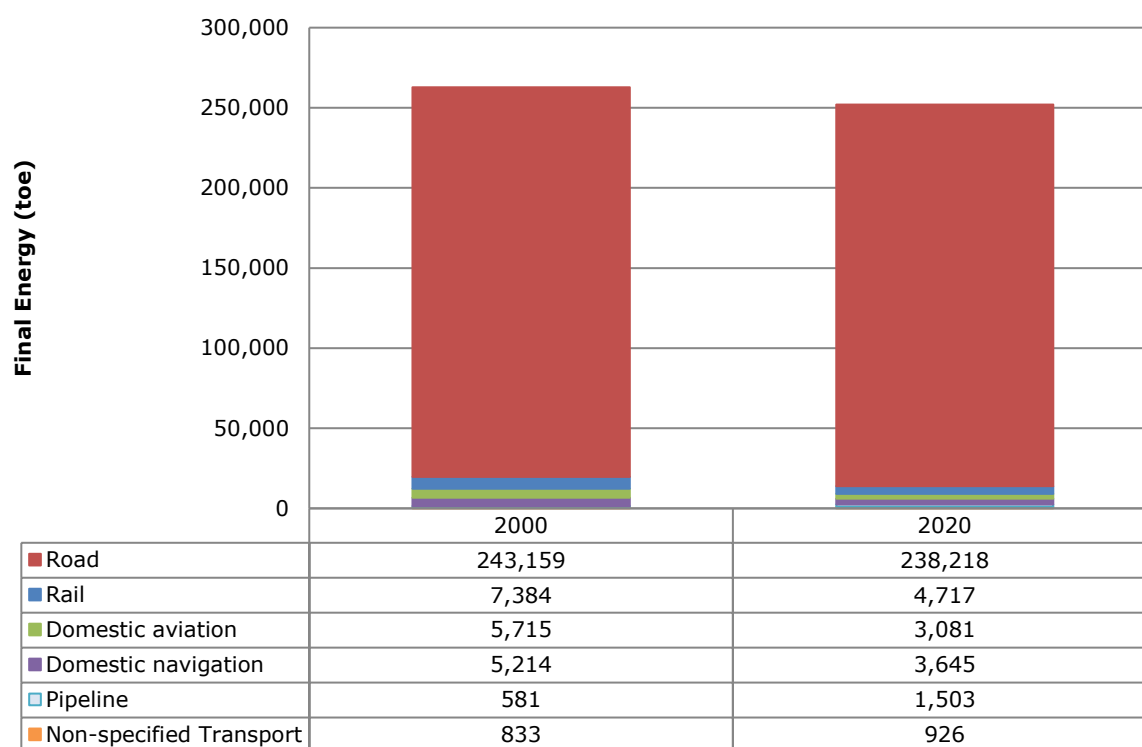
Figure 104: Final energy consumption in the EU-27 by transport mode, 2000 and 2020
