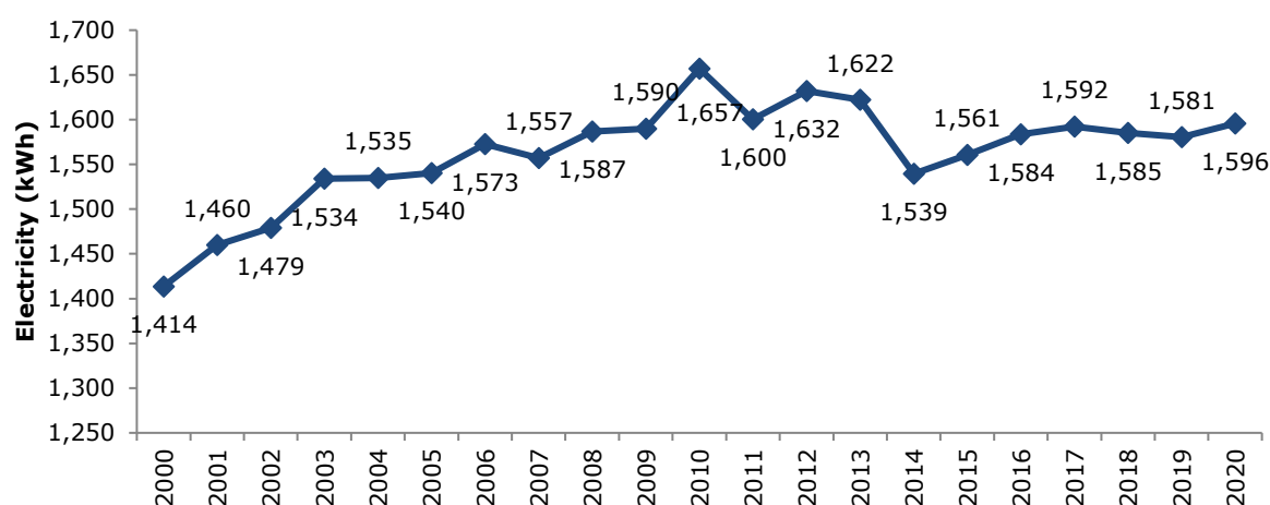
Figure 57: Final residential electricity consumption per capita in the EU-27, 2000-2020
