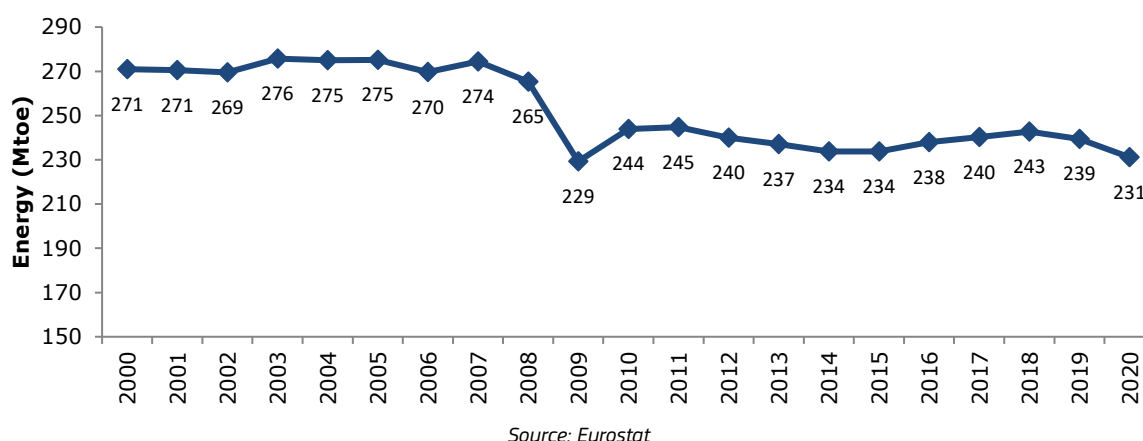
Figure 138: Industry sector: final energy consumption in the EU-27, 2000-2020
