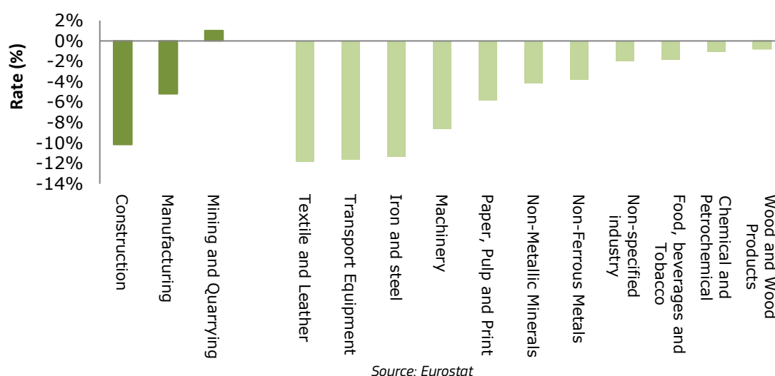
Figure 155: Electricity rates in industrial and manufacturing subsectors in the EU-27, 2019 and 2020
