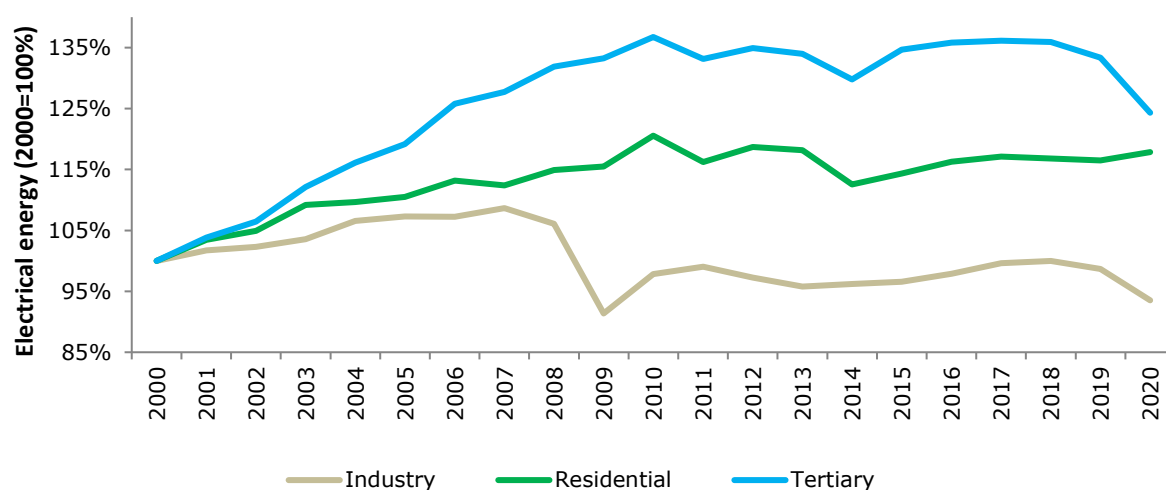
Figure 21: Final electricity Consumption trends of main consuming sectors in the EU-27, 2000-2020 (2000=100%)
