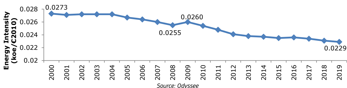
Figure 95: Energy intensity of transport sector in the EU-27, 2000-2019
