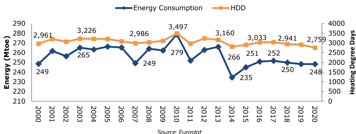
Figure 28: Final residential energy consumption in the EU-27, 2000-2020
