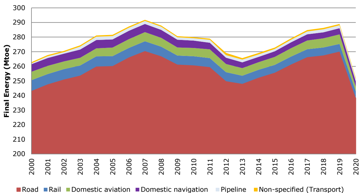
Figure 106: Final energy consumption in the EU-27 by transport mode, 2000-2020
