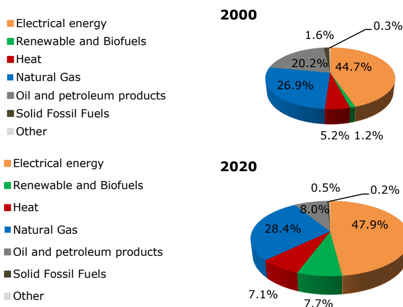
Figure 79: Final energy mix in the tertiary sector in the EU-27, 2000 and 2020
