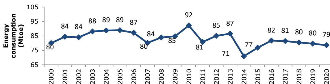
Figure 67: Final residential natural gas consumption trends in the EU-27, 2000-2020
