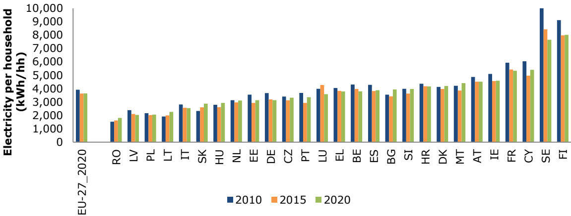
Figure 61: Residential electricity consumption trends per household by Member State in the EU-27; 2010, 2015 and 2020
