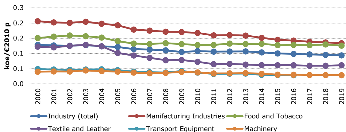
Figure 162: Energy intensity per industry subsector in the EU-27 (GDP at purchasing power parities), 2000-2019 (expanded)
