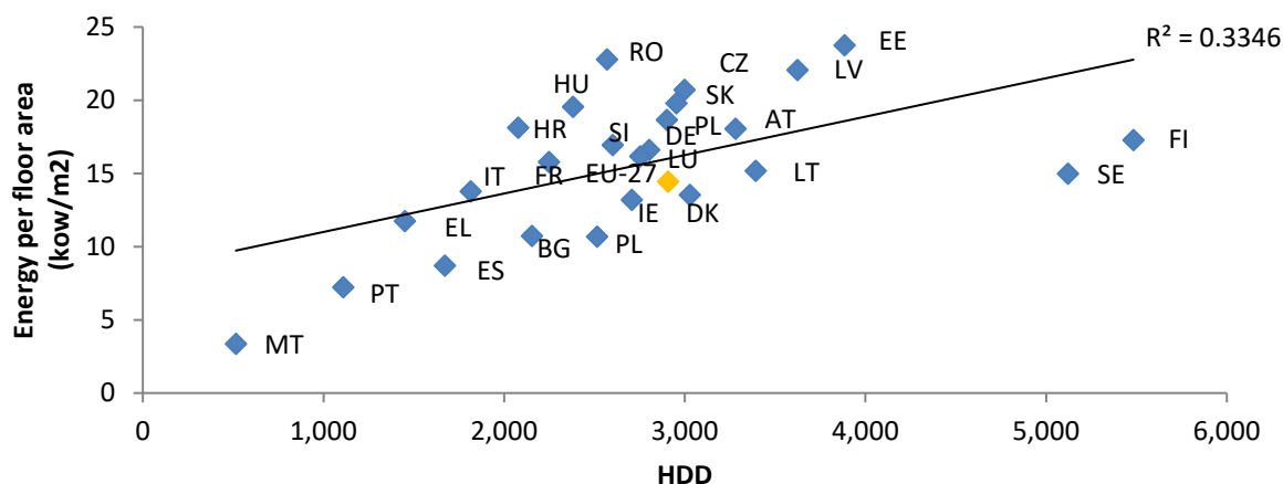
Figure 47: Average energy per unit area climatic corrected 66 vs heating degree days in the EU-27 Member States 67 , year 2019
