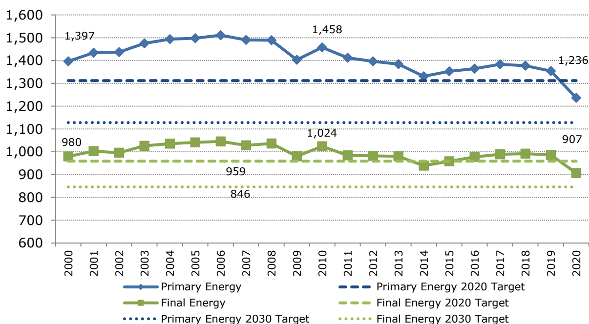
Figure 163: Energy consumption trends with 2020 EU-27 energy targets, 2000-2020
