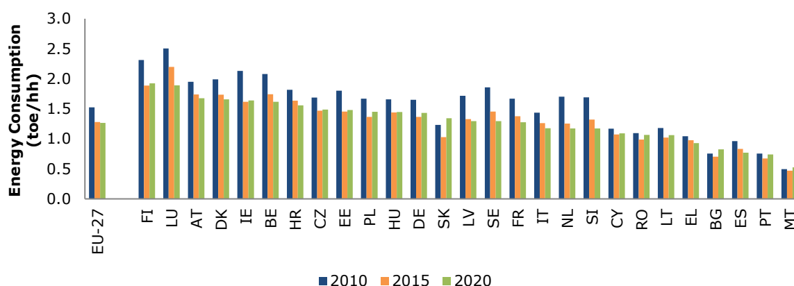
Figure 41: Final Residential energy consumption trends per household in the EU-27 Member States, 2010, 2015 and 2020
