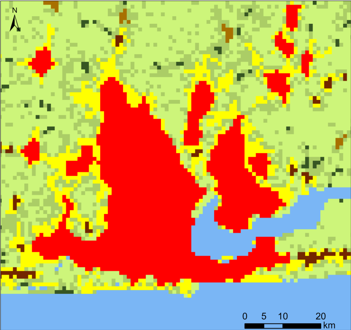
Figure 27 - GHS Settlement Model spatial raster dataset (GHS-SMOD) GHS-SMOD_E2020_GLOBE_R2023A_54009_1K_V1_0 displayed in the area of Lagos (Nigeria) -Legend in Table 21. The boundaries and the names shown on this map do not imply official endorsement or acceptance by the European Union © OpenStreetMap
