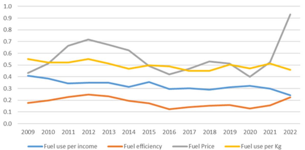
Figure 43 - Change in fuel intensity (l/kg), fuel efficiency (%), fuel use per income generated (l/EUR) and fuel price, 2009–2022
