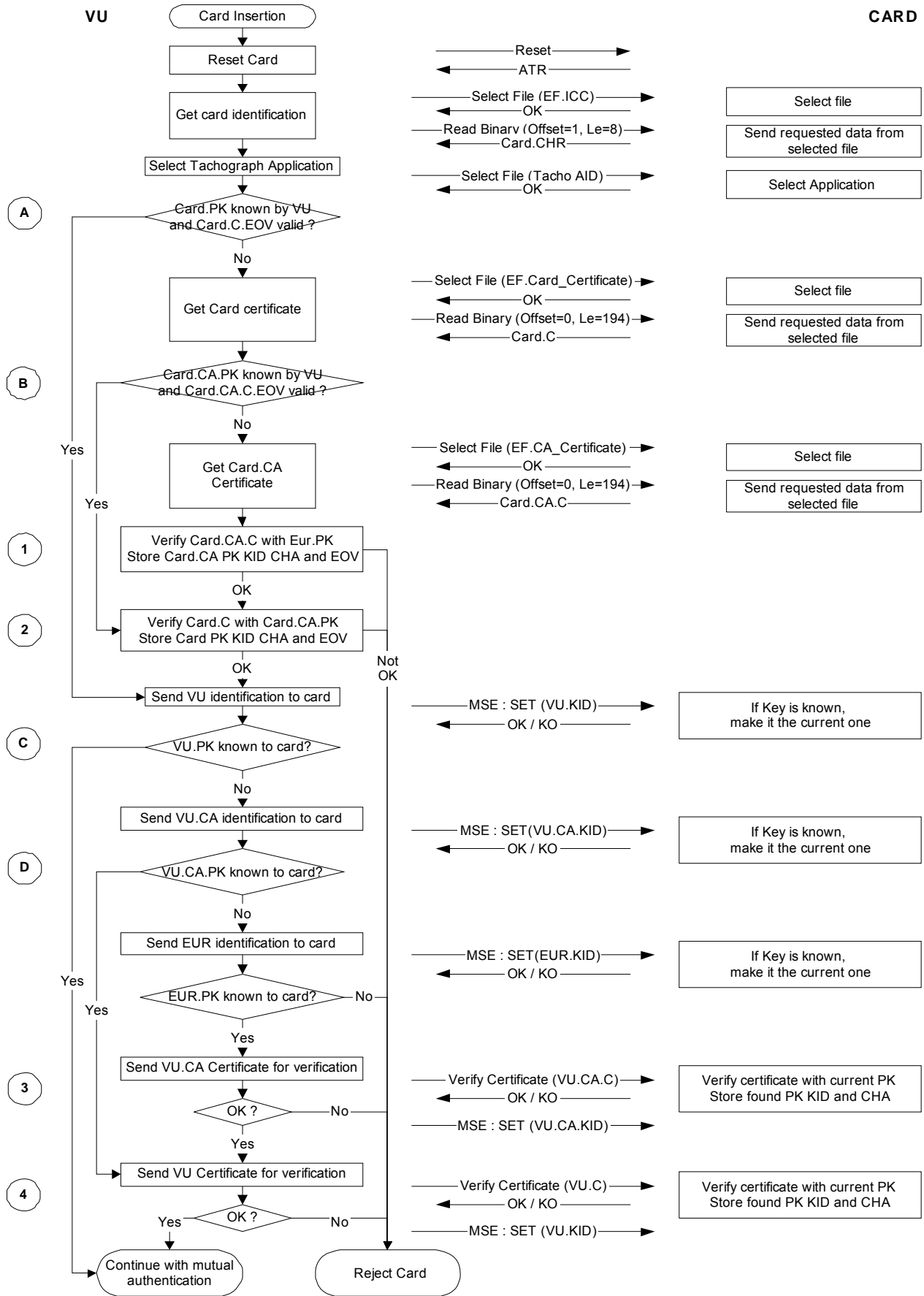
Figure 9.1: Annex I(B) Appendix 11 CSM_020 mutual authentication protocol
