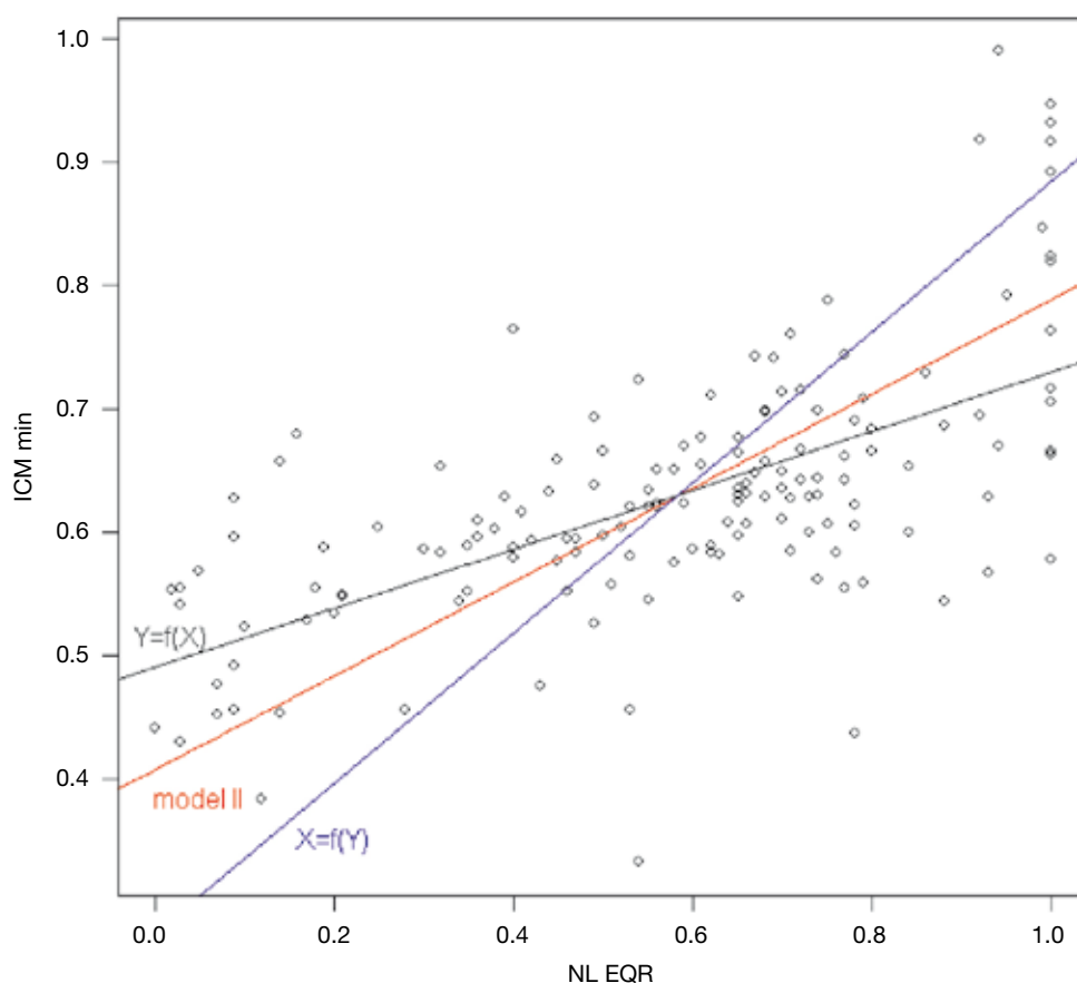
Figure 2.2.9: Model I and model II regression equations for the Dutch dataset used in the phytobenthos intercalibration exercise. In model I regression, the sum of vertical squared deviations is minimised when regressing Y on X; the same thing occurs horizontally when regressing X on Y. In model II regression, the sum of squared Euclidian distances to the regression line is minimised. Fitted results are the same from X to Y as well as from Y to X with a model II regression; this is not the case for model I (generally).
