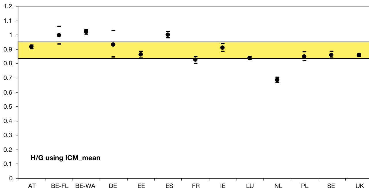
Figure 2.2.16: High / good boundaries proposed by participants in the CB GIG phytobenthos intercalibration exercise. Data points show either the predicted boundary value \pm 95% confidence limits (for those countries with a single H/G boundary value) or the median of all national boundary values, along with the highest and lowest confidence limits of the predictions (for those countries with >1 H/G boundary value. The blue rectangle shows the approximate limits of acceptable boundary values: 0.839 – 0.939.
