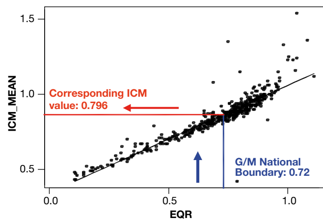
Figure 2.2.14: Conversion of the Good/Moderate national boundary value for a hypothetical national dataset into an ICM value using the regression shown in Fig. 2.2.13.
