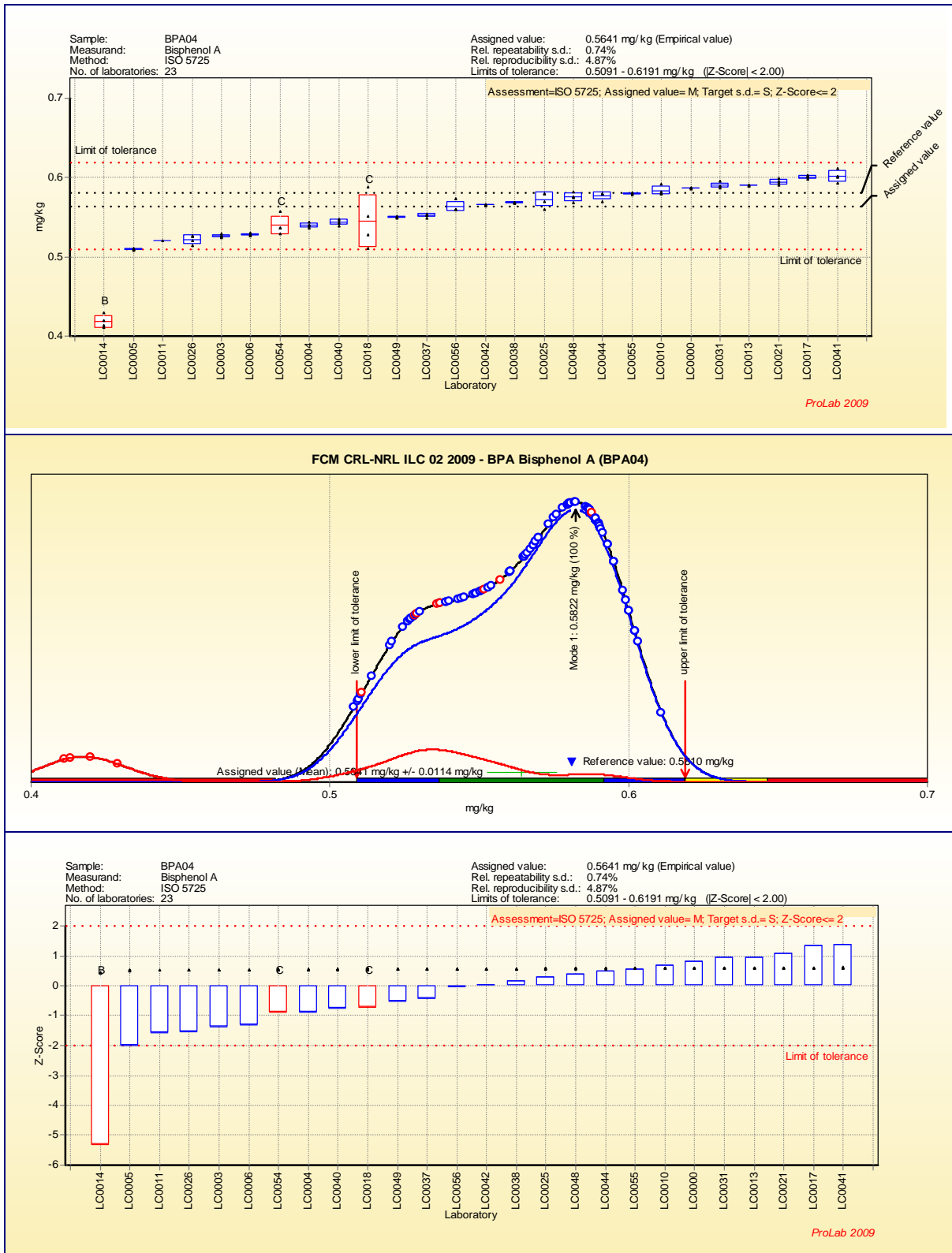
Figure 2d: Summary graphs of the laboratory's test results with their repeatability SD (a), Kernel Density plot (b) and z-scores (c)
