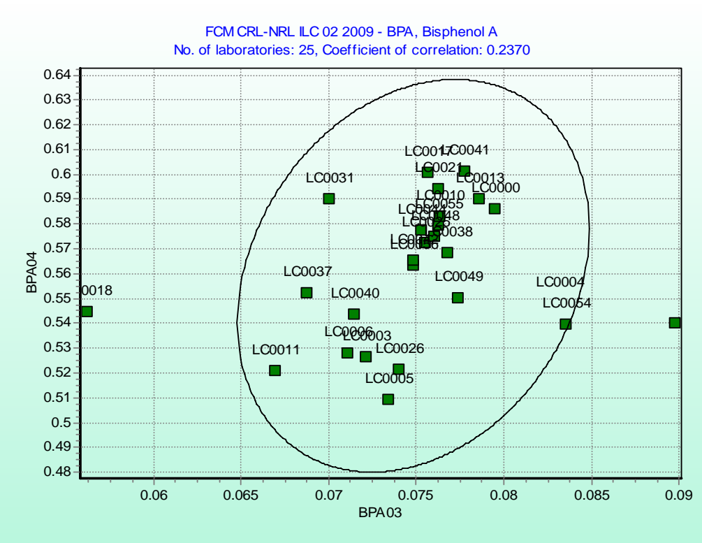
Figure 6 b - Yoden plot BPA03 against BPA04 –in high level calibration range
