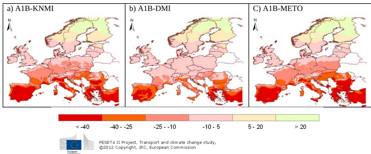
Figure 18: Vulnerability to rail track buckling: Changes in period suitable for maintenance by 2070-2100 as compared with 1990-2010 for scenarios A1B (number of days in a year)
