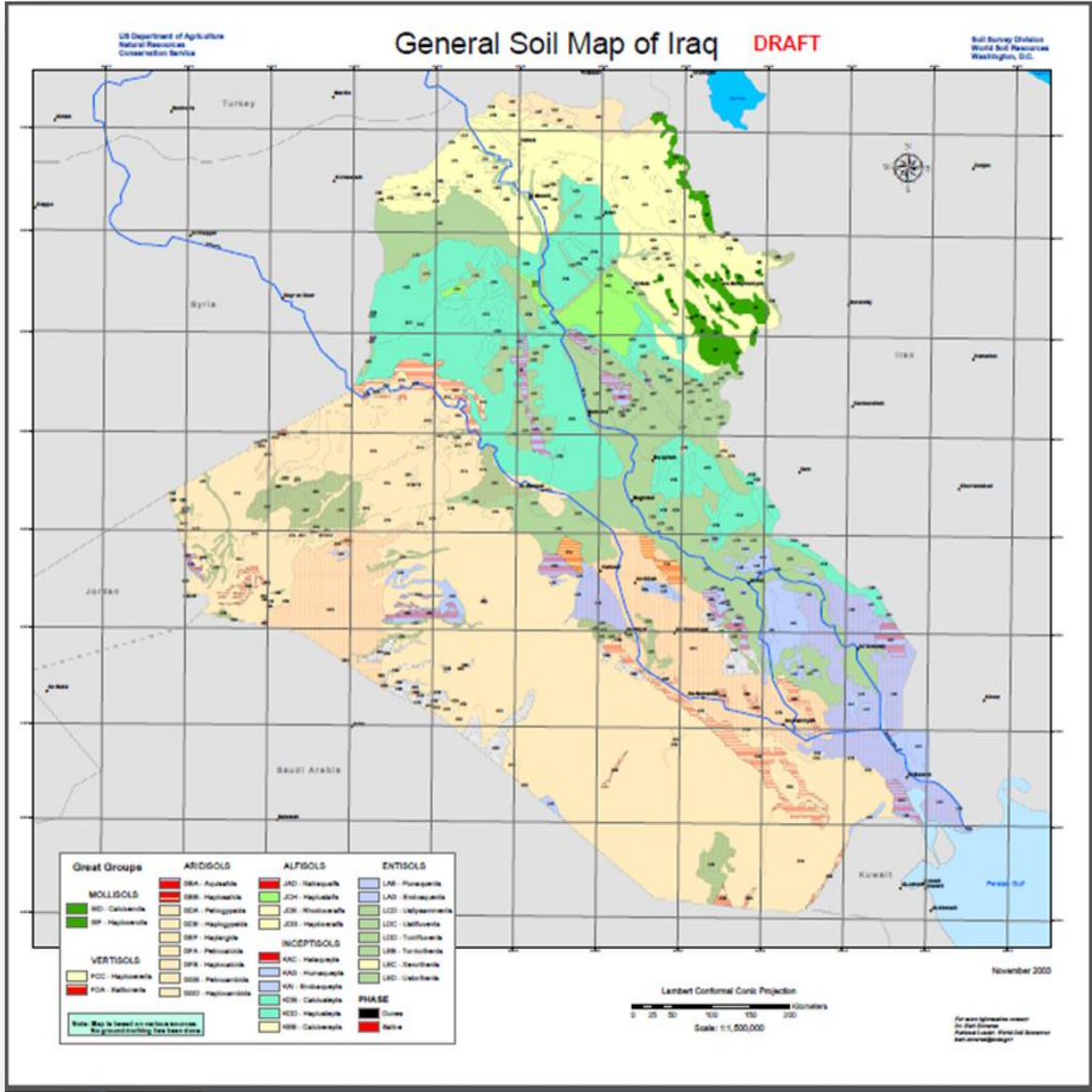
Figure 3. General Soil map of Iraq
