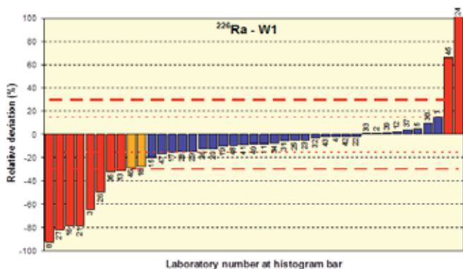
Results of the monitoring laboratories for the determination of 226 Ra in mineral water.
