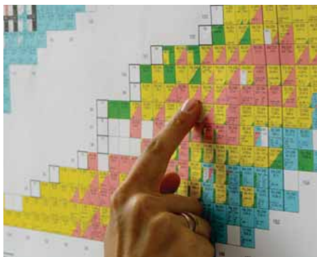
The Karlsruhe nuclide chart.
